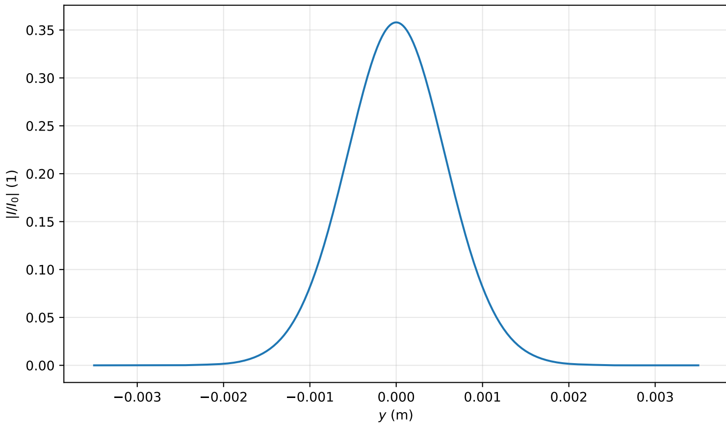
Intensity profile I(x=0, y, z=3.105)/I_0 , P_{in}=0.2P_{cr} , artificial time
